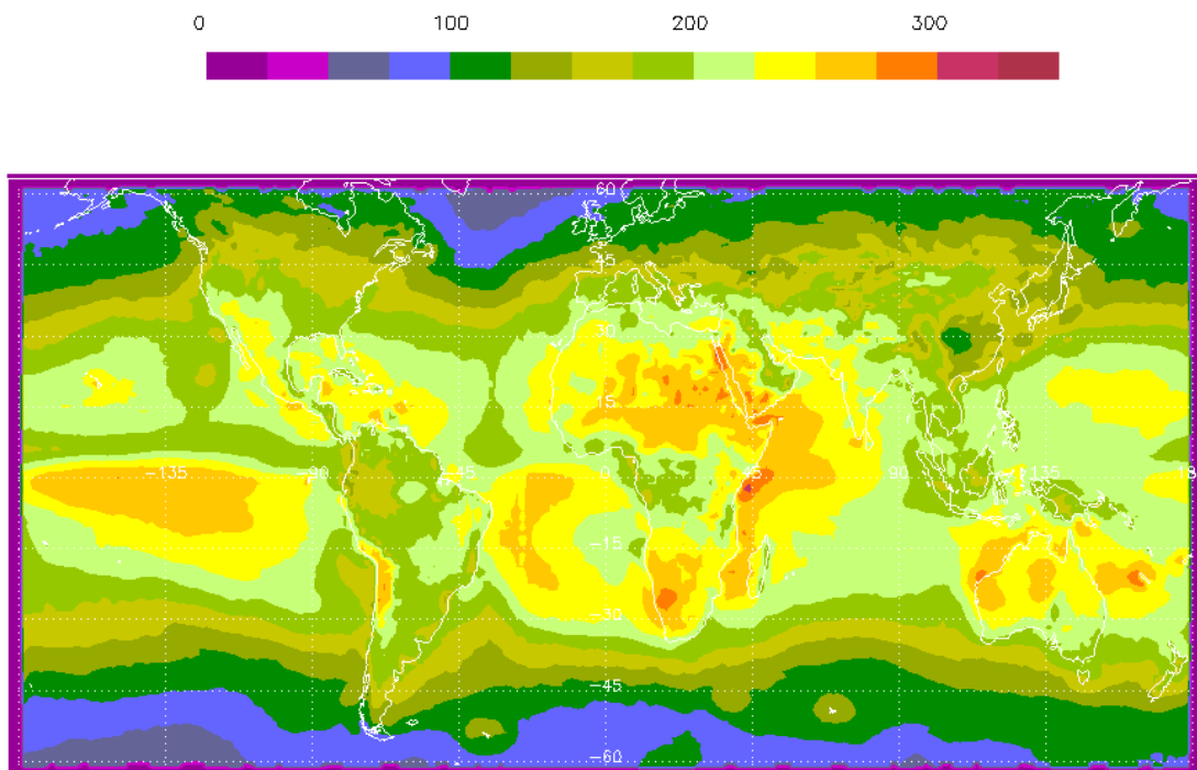
Fig. 3.1.1: Global irradiance map for January in W/m^2 based on satellite and ground information. Means adopted mainly to 1981–2000.
